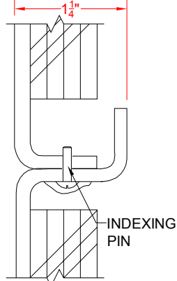
SECTION E - E - SCALE: NTS WALL JOINT DETAIL
