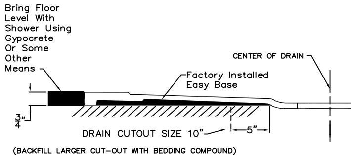
CROSS-SECTION OF THRESHOLD
